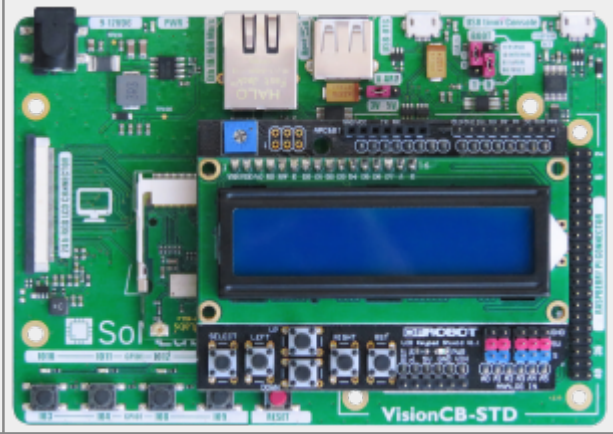
VisionCB-STD v2.0 board with Arduino Shield
